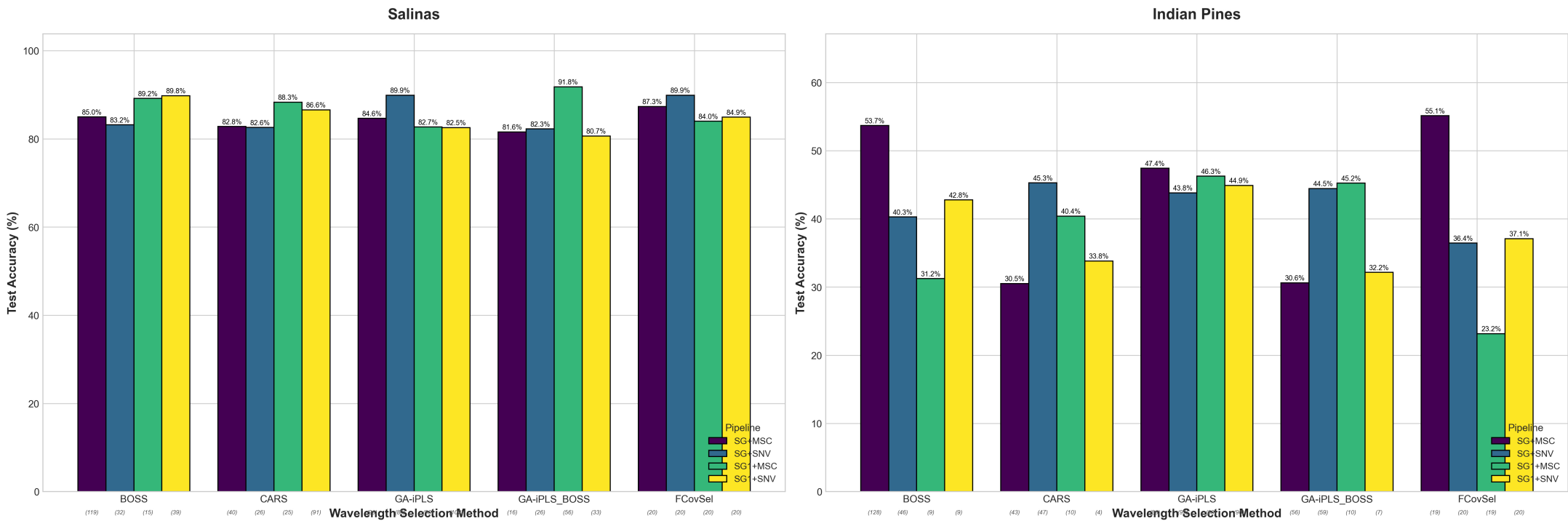
3D-CNN Test Accuracy by Wavelength Selection Method & Preprocessing (Number of selected bands shown in parentheses)
